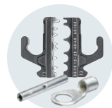
Crimping die 97 39 13: Crimps connections for uninsulated cable connectors from 0.5 – 10 mm 2
